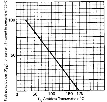
FIG. 3. Derating curve
